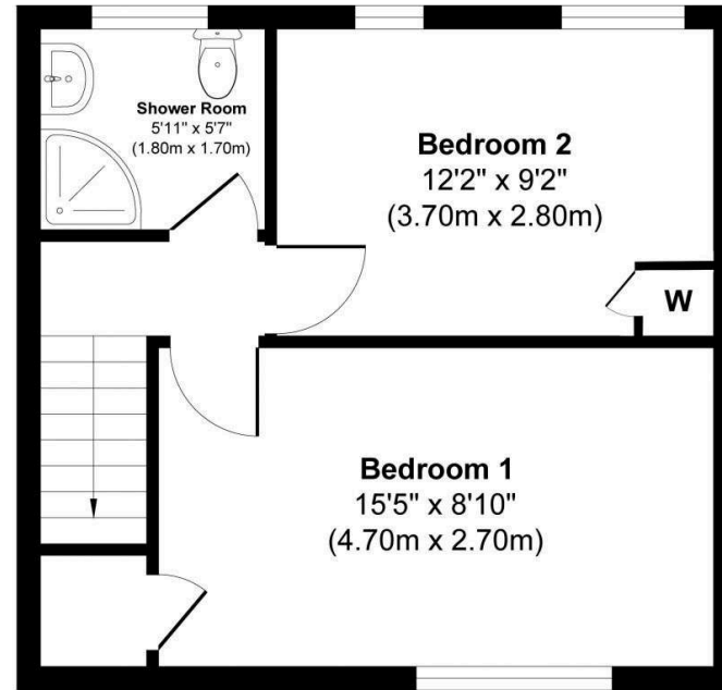
First Floor Approximate Floor Area 331 sq. ft (30.78 sq. m)
